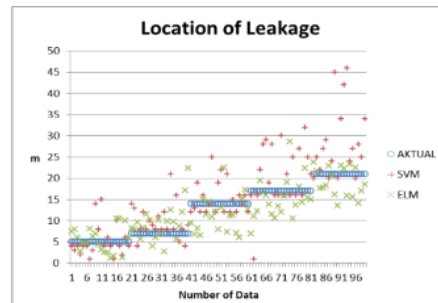
Figure 5 : Prediction of location and magnitude of leakage in pipe 1138
